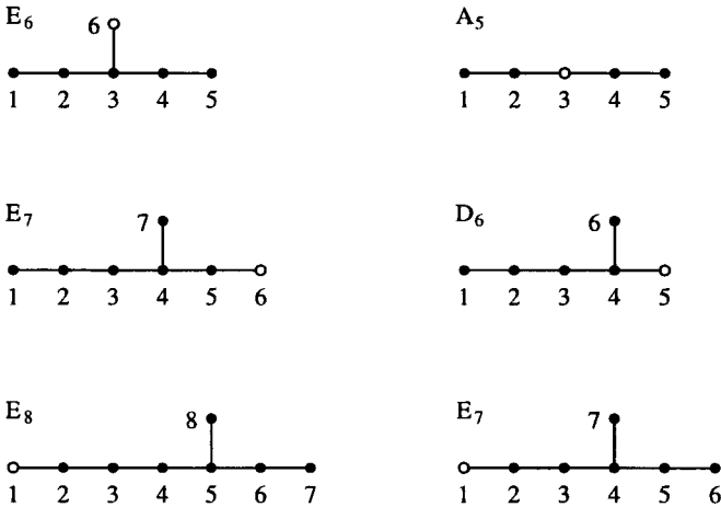
Fig. 1. Dynkin diagrams of the Lie algebras E_n , A_5 and D_6 with labelling of vertices as used in the text. Removing the marked vertex (and its corresponding edge) in a diagram of the first column yields the diagram to its right. Conversely, adding a vertex plus edge to the marked vertices in the second column yields the graphs of the first column.
